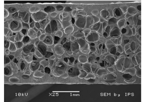
SEM Image of closed-cell foam
